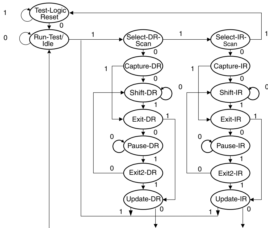
Figure 12 • TAP Controller State Diagram
